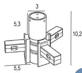
T-LOW SPACER 3
