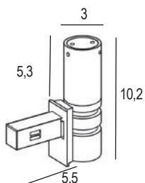
T-LOW SPACER 1
